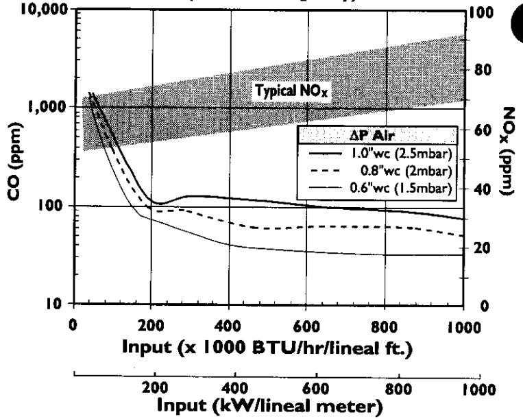
NO x and CO Emission Data (at 3 vol. % O 2 - dry)
