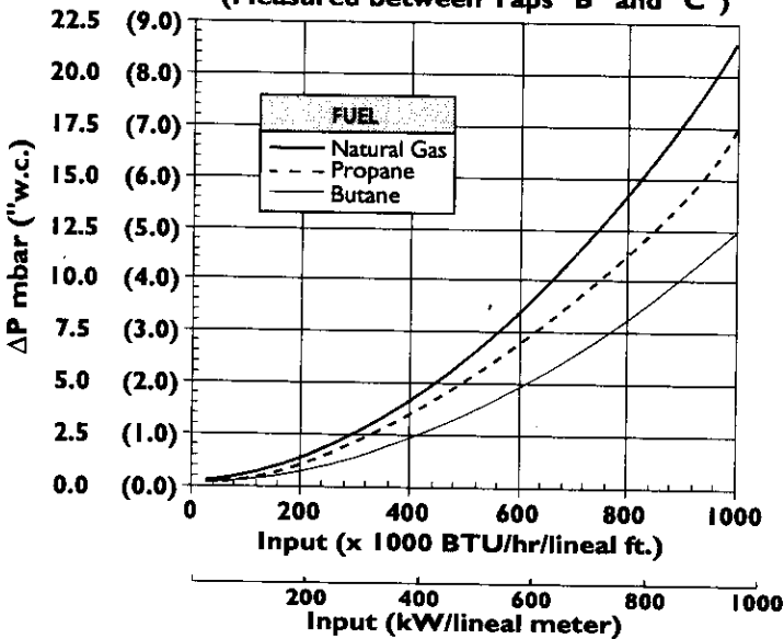
Fuel \Delta P vs. Input (Measured between Taps "B" and "C")
